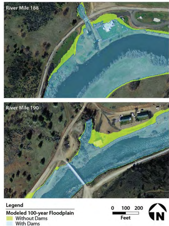
Figure 4.2-23: Close up of one or two structures potentially affected by the change in the 100-year floodplain – comparison of dams in and dams out floodplain. (NOT A REGULATORY FLOOD PLAIN, this is just a comparison)
